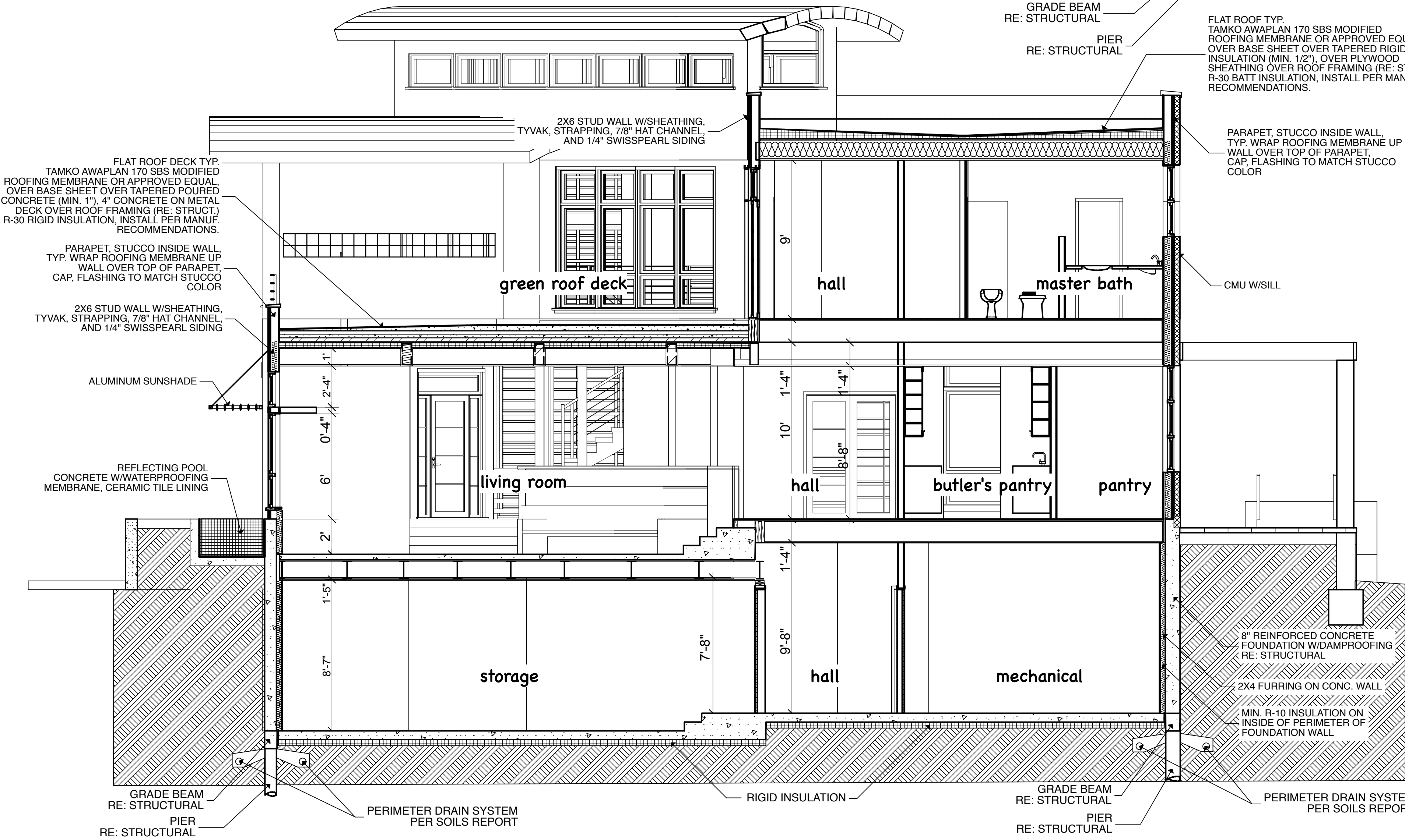
NORTH-SOUTH SECTION S-1 scale: 1/4" = 1'-0"
