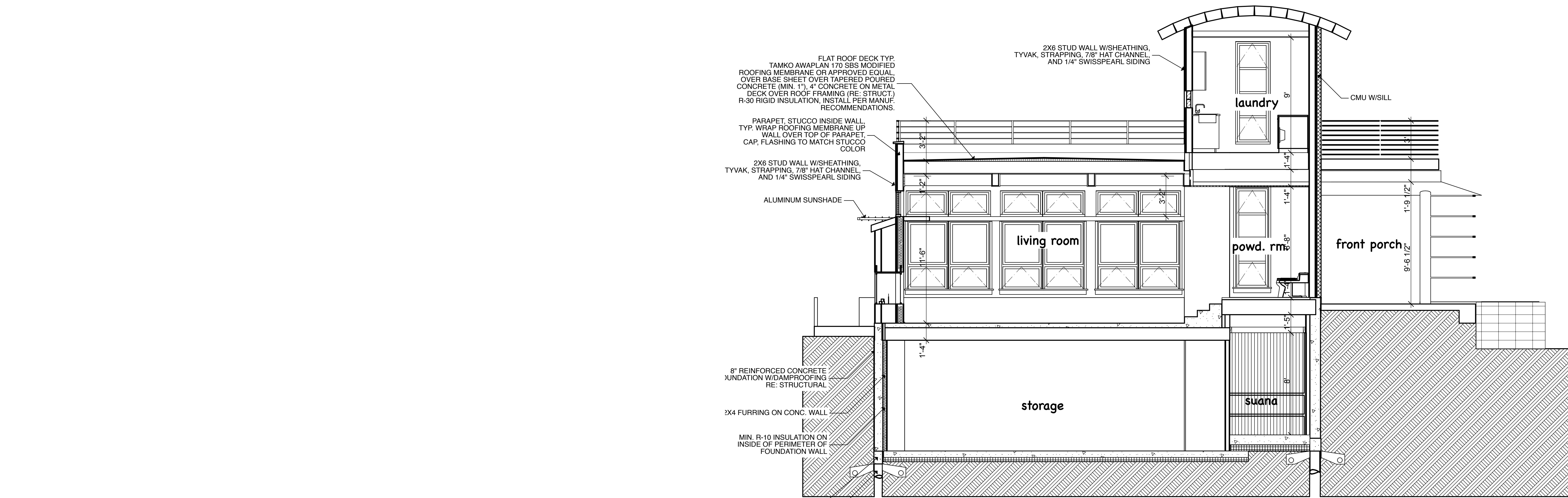
EAST-WEST SECTION S-2 scale: 1/4" = 1'-0"
